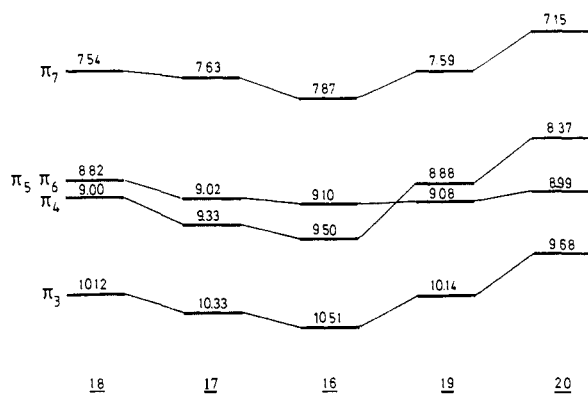
Figure 2. Energy level diagram for trans -stilbene ( 16 ) and several para-substituted trans -stilbenes.
