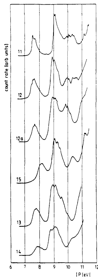
Figure 3. Low energy part of the UP spectrum of cis -stilbene ( 15 ) and several 1,2-diphenylcycloalkenes.
