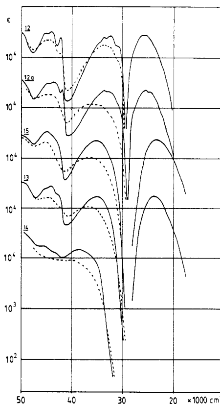
Figure 5. Electronic spectra of cis -stilbene ( 15 ) and several 1,2-diphenylcycloalkenes: (---) absorption spectrum at room temperature, (—) absorption and emission spectra at liquid nitrogen temperature.
