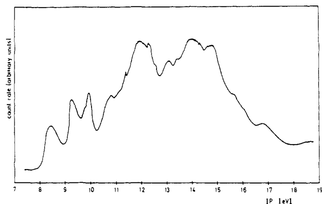
Figure 1. UP spectra of 1-phenylcyclohexene ( 10 ). See Table III for energies of band maxima.
