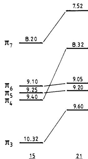
Figure 4. Energy level diagram for cis -stilbene ( 15 ) and p,p' -dimethoxy- cis -stilbene ( 21 ).
